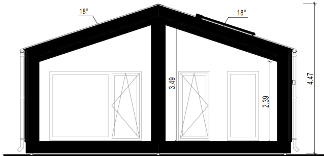
A SECTION 1:80
